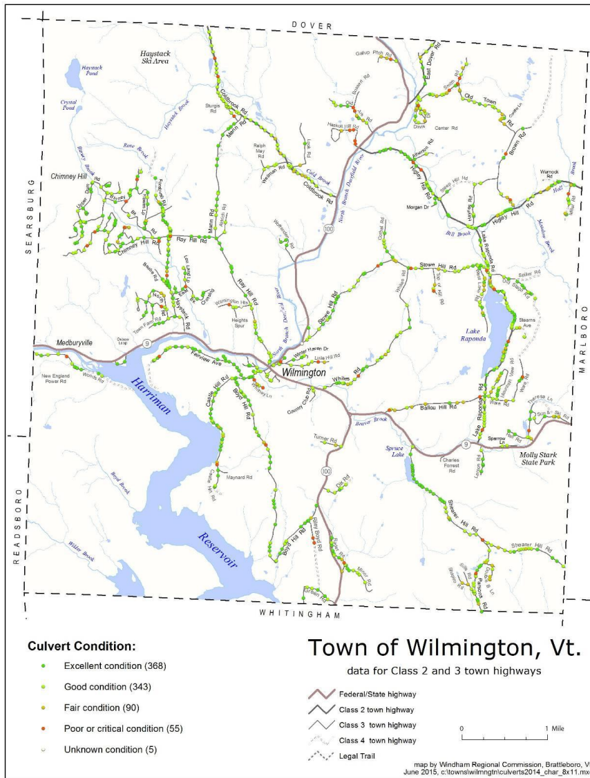
Figure 55: Culverts by Condition
