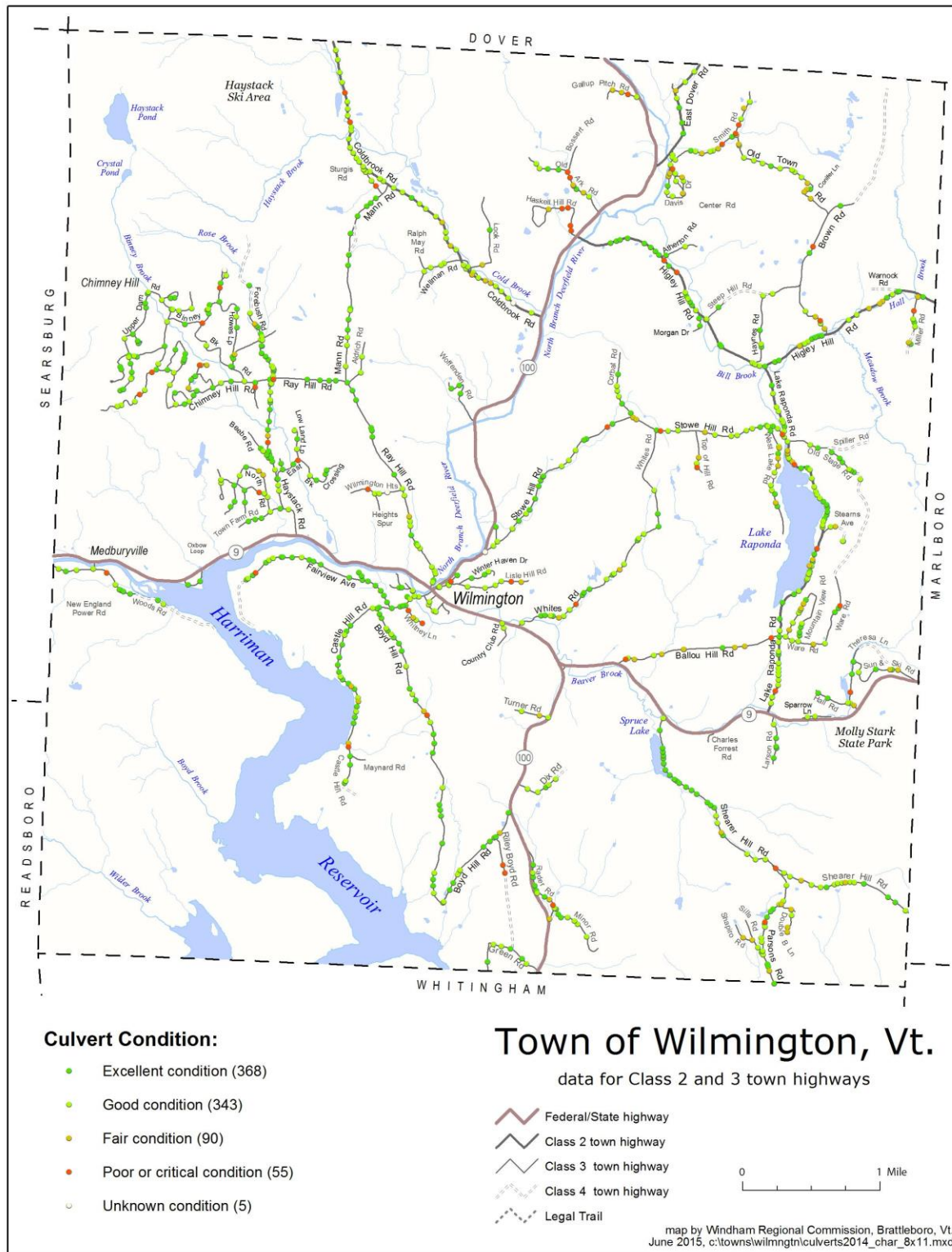
Figure 47: Culverts by Condition
